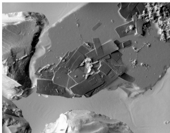
Fig. 12. A10 (silica with diethylenetriamino functional groups) composite loaded with lanthanum at pH 2.
