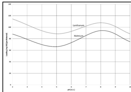
Fig.1.Loading over altering pH on silica-based resin.
