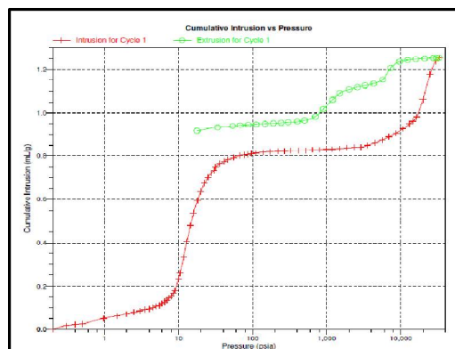
Fig. 3.Cumulative intrusion of mercury in unloaded silica/amine resin.
