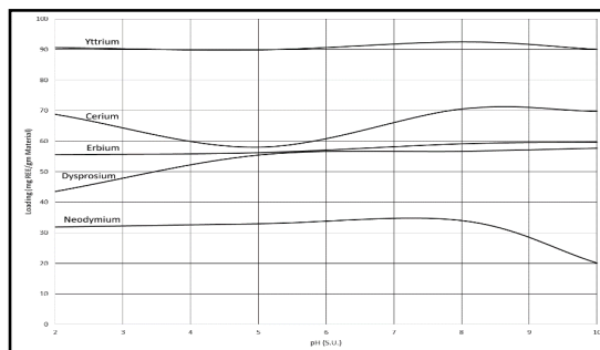
Fig.2. Loading over altering pH on polystyrene-based resin.
